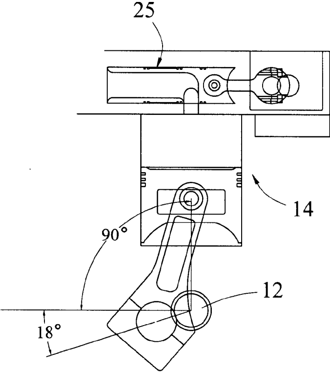
Intake Valve Open at 108°
