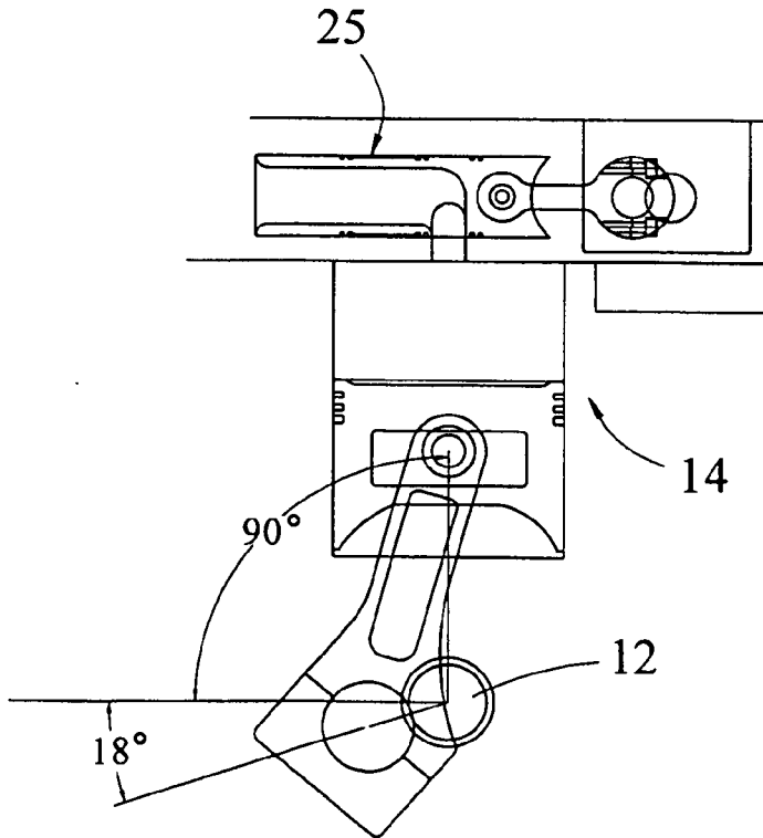
Intake Valve Open at 108°
