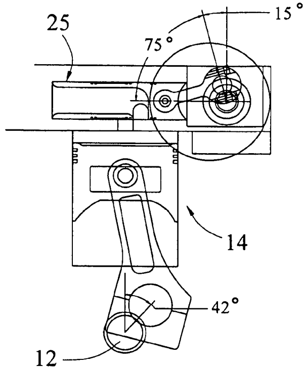
Beginning of Intake Stroke
